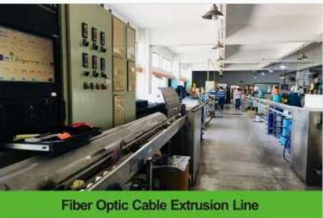
Fiber Optic Cable Extrusion Line
