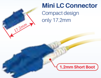
LC Duplex SLL Connector
