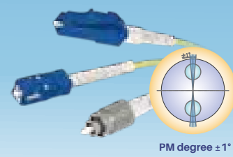
PM optical fiber connector
