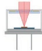
Hermetical TO-lens package
