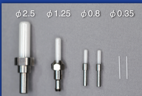
Extra Fine Ferrules
