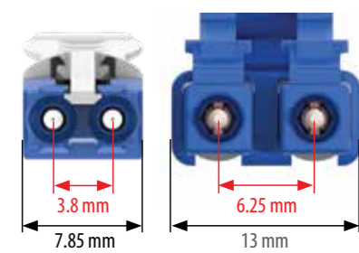
CS Connector LC Duplex
